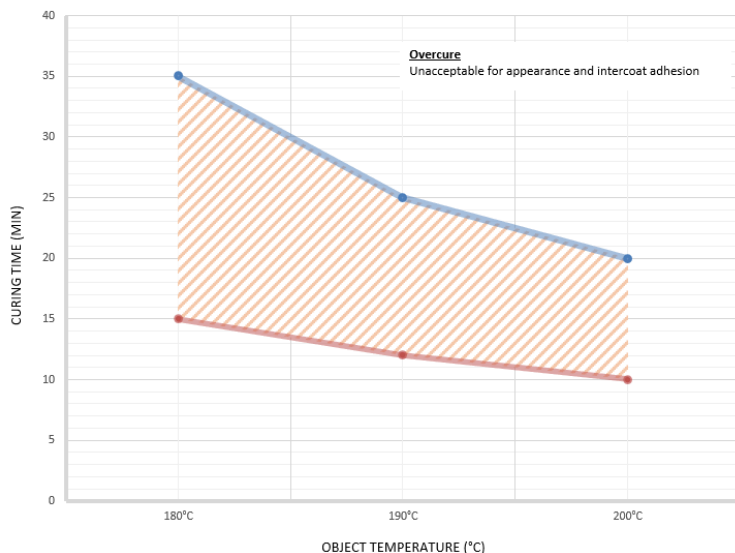
Interpon D2525 Matt AM - curing window
