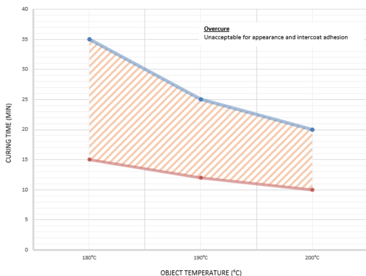
Interpon D2525 Structura Flex - curing window
