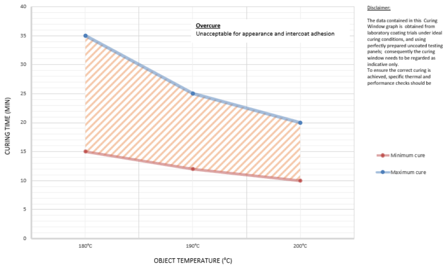
Interpon D2525 Texture AM - curing window
