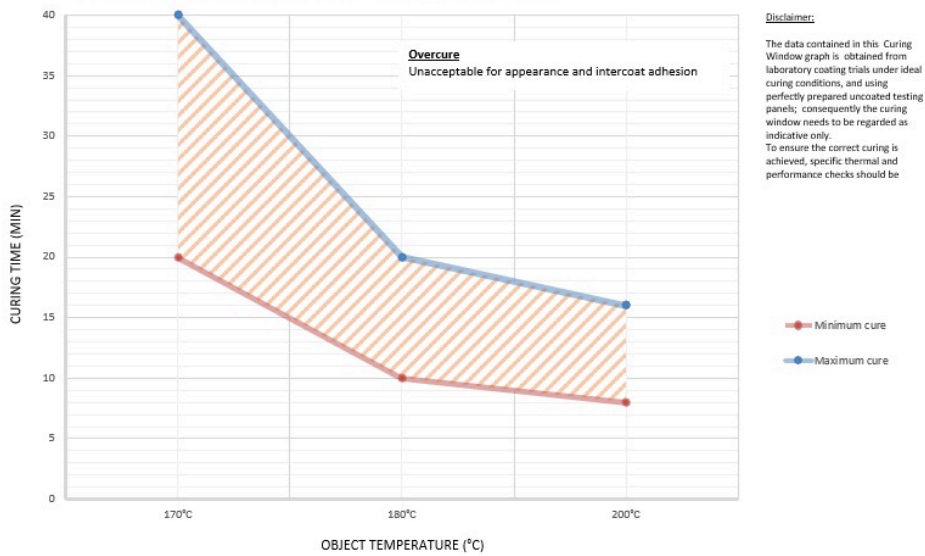
Interpon D1036 Gloss AM - curing window
