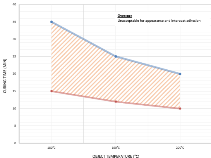
Interpon D2525 Matt X-Pro - curing window
