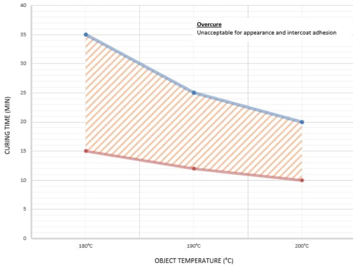
Interpon D2525 Structura - curing window
