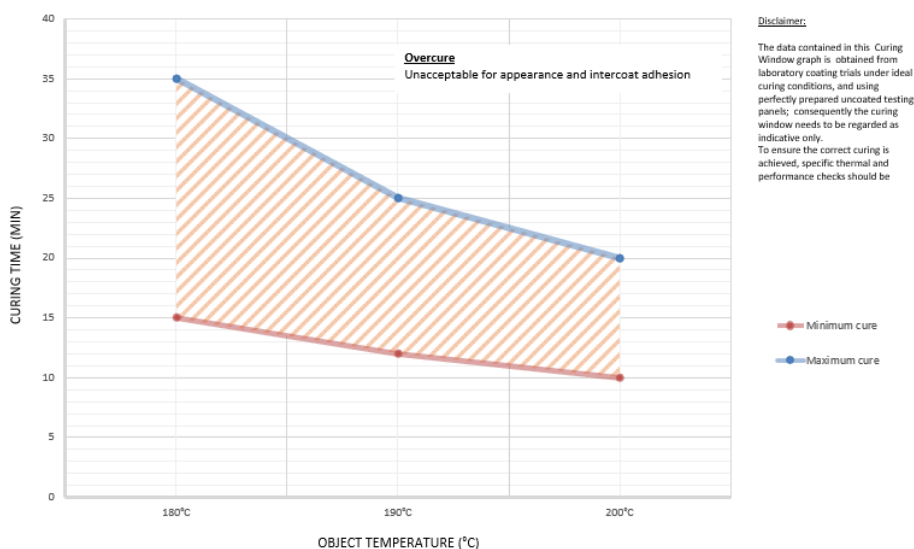
Interpon D2525 Matt Flex - curing window
