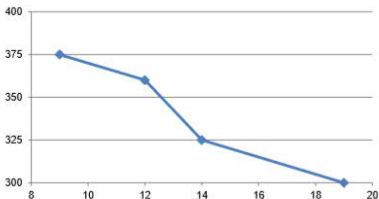
Cure Window - Temp (Deg F) v Time (min)
