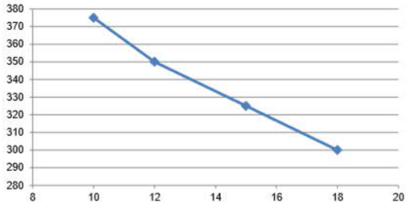
Cure Window - Temp (Deg F) v Time (min)
