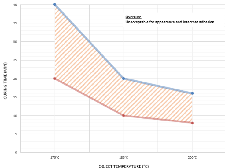
Interpon D1036 Satin X-Pro - curing window
