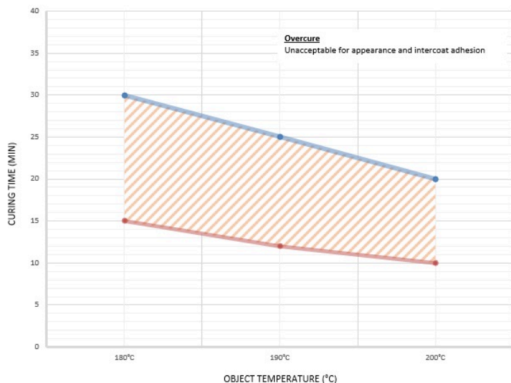
Interpon D1036 Matt X-Pro - curing window
