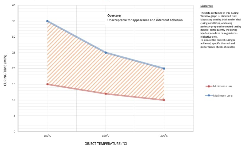
Interpon D2525 Sable - curing window
