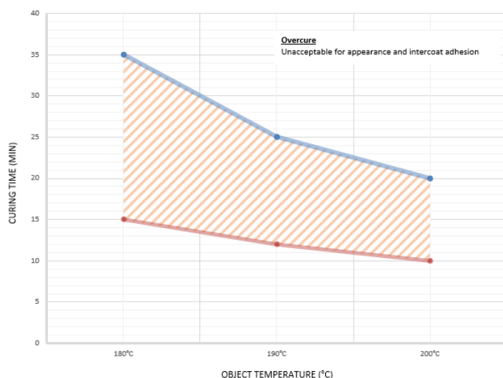
Interpon D2525 Satin - curing window
