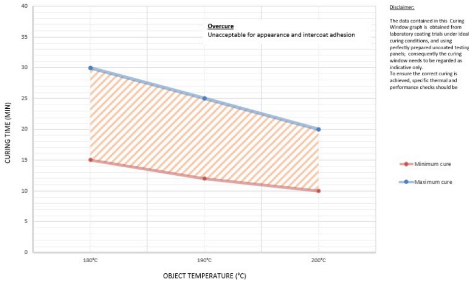
Interpon D1036 Matt X-Pro - curing window
