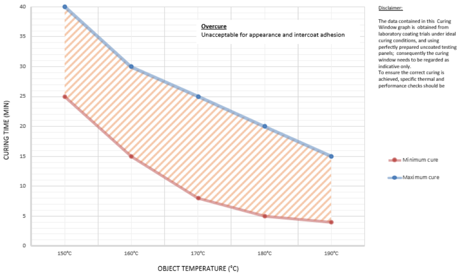
Interpon D1036 Low- E Texture - curing window
