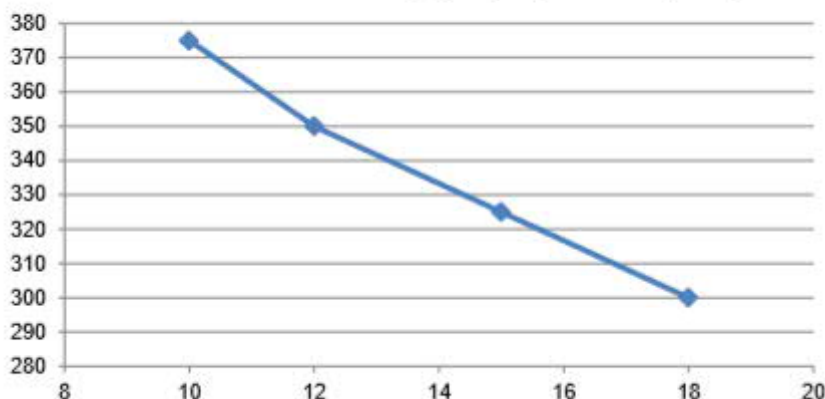
Cure Window - Temp (Deg F) v Time (min)
