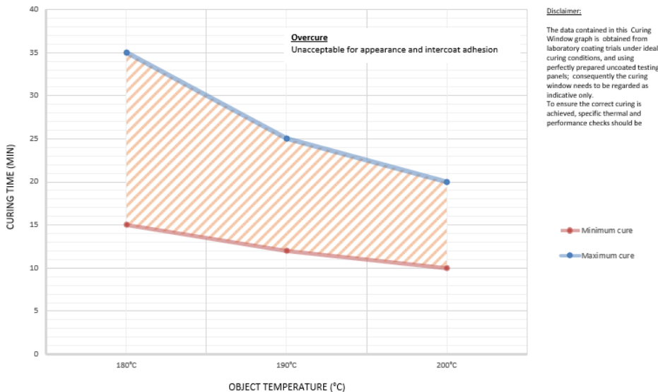
Interpon D2525 Sable - curing window
