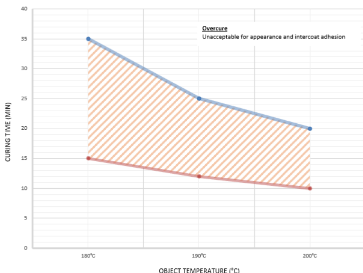
Interpon D2525 Texture - curing window
