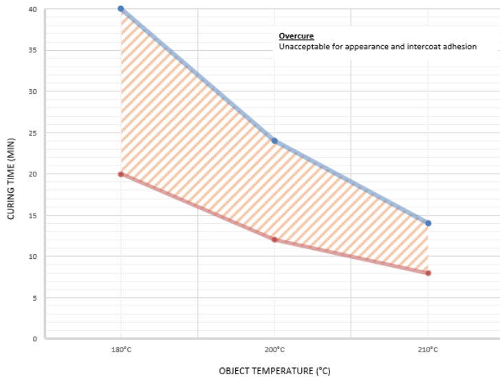
Interpon D1036 Texture AM - curing window
