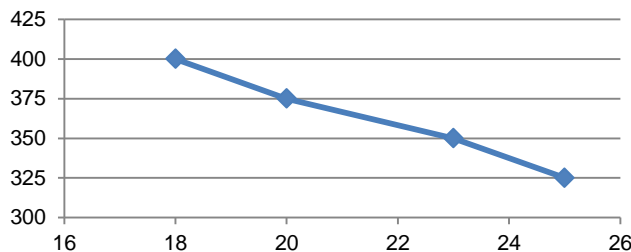
Cure Window - Temp (Deg F) v Time (min)
