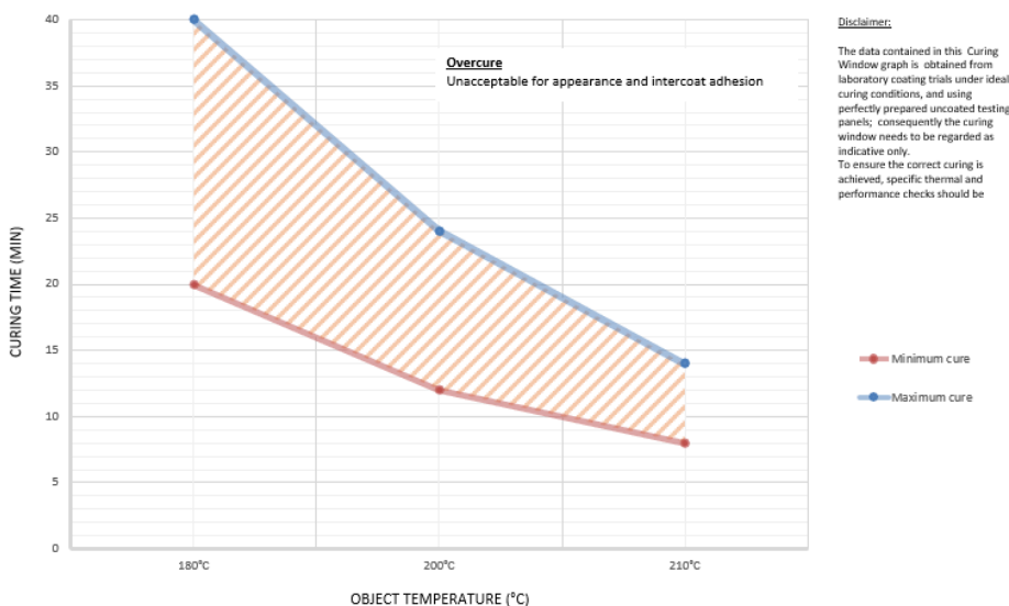
Interpon D1036 Texture - curing window
