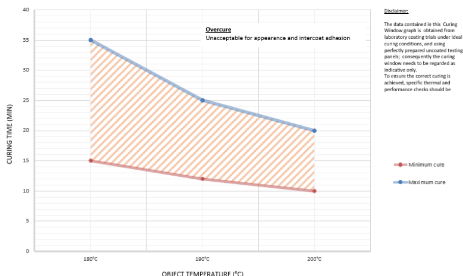
Interpon D2525 Matt X-Pro - curing window
