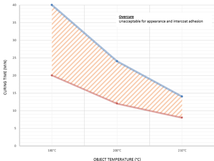
Interpon D1036 Sable - curing window
