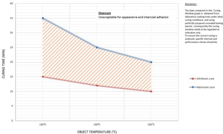
Interpon D2525 Matt - curing window
