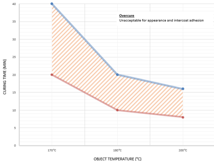
Interpon D1036 Satin X-Pro - curing window
