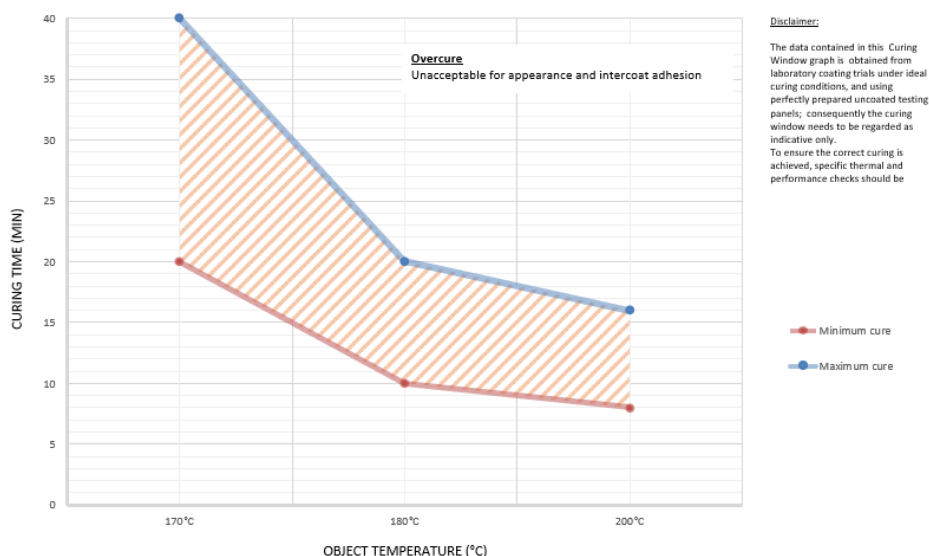
Interpon D1036 Satin X-Pro - curing window
