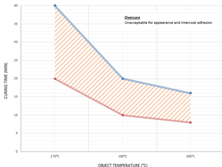
Interpon D1036 Satin - curing window
